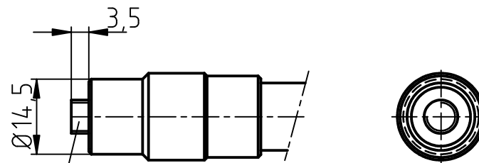
Conector SMAH (SMAF)
