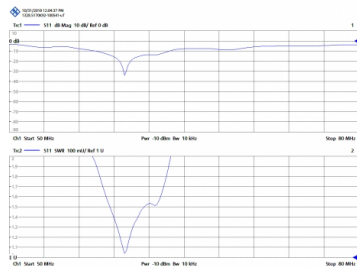
Conical rod
