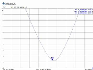
Two segment antenna
