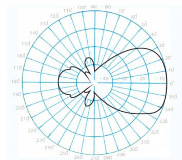
Vertical radiation pattern
