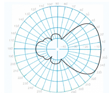
Horizontal radiation pattern
