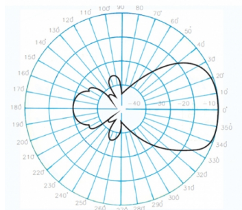
Vertical radiation pattern
